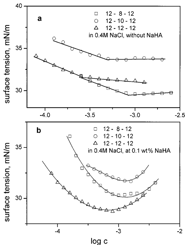
FIG. 1. Surface tension of NaCl–12- s -12 dimeric surfactant system in aqueous 0.40 M NaCl solution vs \log c at different surfactant structures (variable parameter s ). (a) Without NaHA. (b) With 0.1 wt% NaHA.
