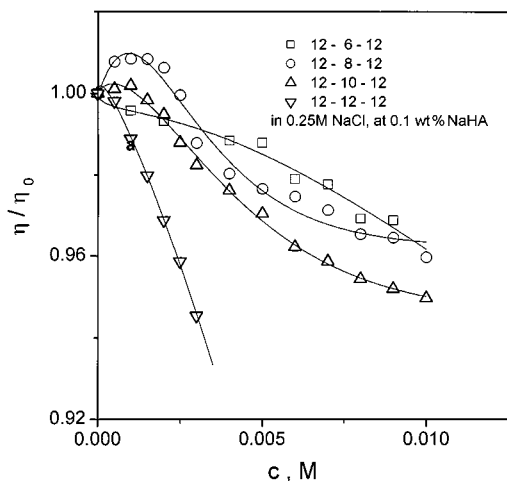
FIG. 4. Relative viscosity \eta/\eta_0 of 0.1 wt% NaHA–NaCl–12- s -12 dimeric surfactant system in aqueous 0.25 M NaCl solution vs surfactant concentration c at different surfactant structures (variable parameter s ). \eta_0 means viscosity of NaHA in 0.25 M NaCl solution at zero surfactant concentration.
