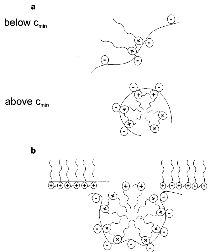
FIG. 5. Model of the NaHA–dimeric surfactant interaction: (a) in solution, (b) at interface.
