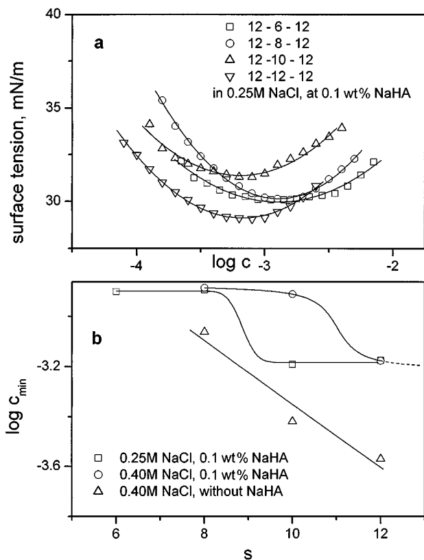
FIG. 2. (a) Surface tension of 0.1 wt% NaHA-NaCl-12- s -12 dimeric surfactant system in aqueous 0.25 M NaCl solution vs \log c at different surfactant structures (variable parameter s ). (b) Plot of \log c_{\min} obtained from Figs. 1b and 2a vs parameter s . The cmc of 0.40 M NaCl-12- s -12 dimeric surfactant system without NaHA is included as symbol \Delta .
